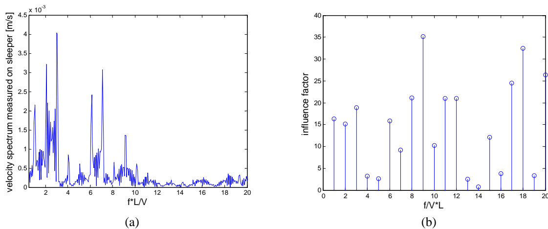
Figure 3: (a) Velocity spectrum as a function of the frequency normalized by V/L , (b) Influence factors at the normalized trainload dominant frequencies.
