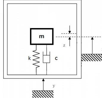
Figure 4: Linear single degree-of-freedom base excited system.
